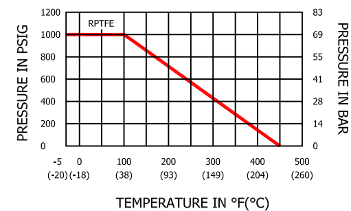
Pressure VS. Temperature Chart
